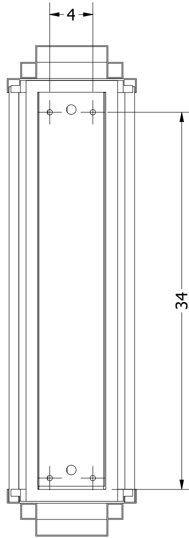
Backplate
